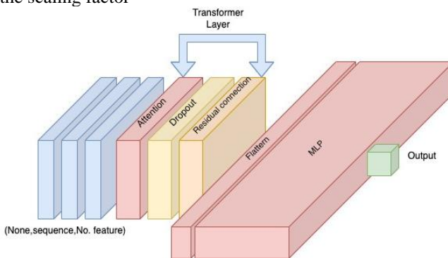
Fig. 7 The architecture of transformer-based model
