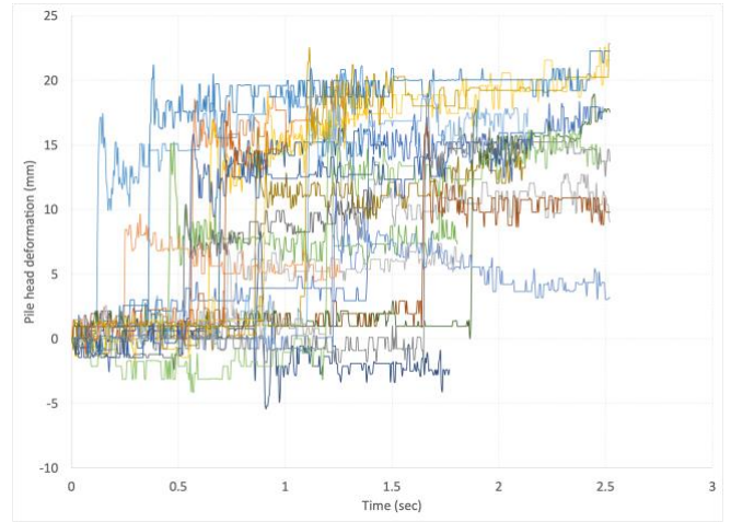
Fig. 6 Pile head deformation from ArUco target
