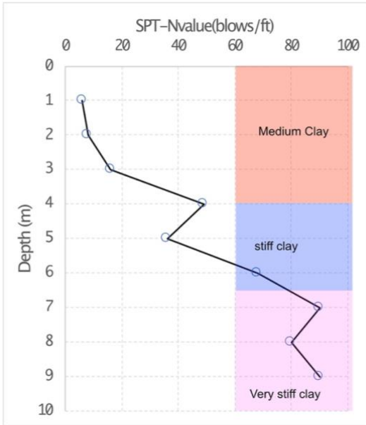
Fig. 4 The value of SPT-N value VS Depth
