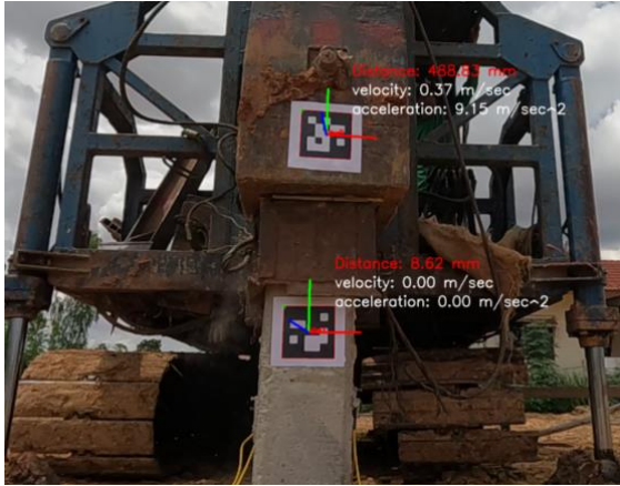
Fig. 3 The ARUCO target installation during testing
